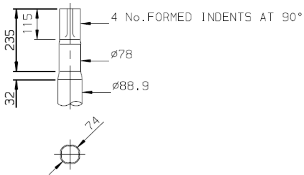
DETAIL OF TOP OF COLUMN.
